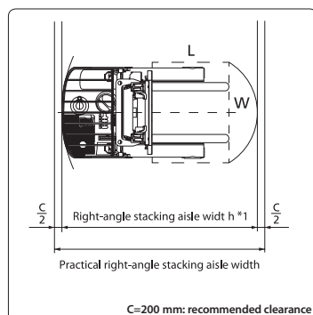
Right angle stacking aisle width
