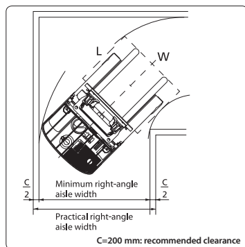
Minimum right angle aisle width
