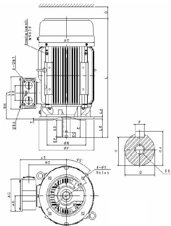
Figure 7-25: Outline drawing of cast iron design, mounting V1; frame size 180
