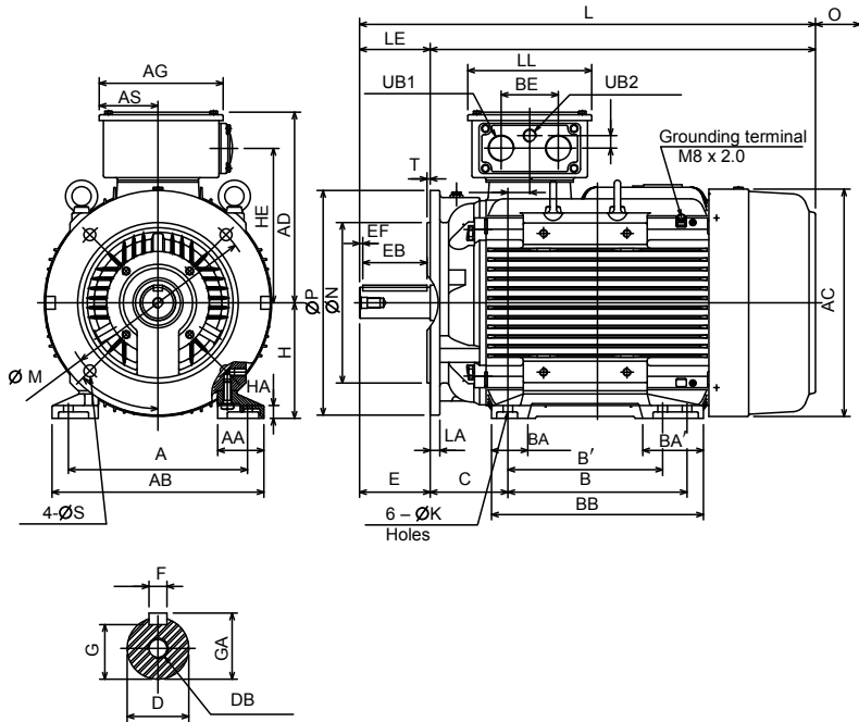
Figure 7-18: Outline drawing of cast iron design, mounting B35; frame size 160 – 180
